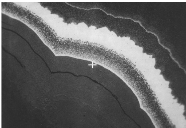
Figure 20. Back-scatter electron image of "allemontite" consisting of an intimate intergrowth of 95% stibarsen and 5% arsenic in the light colored bands and 50% stibarsen/50% arsenic in the gray bands. U.B.C. collection; Mark Mauthner photo.
