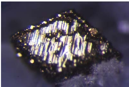
Figure 7. Arsenopyrite crystal, 0.8 mm, with löllingite. Mark Mauthner collection and photo.
